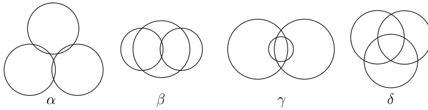
Fig. 1. Arrangements of three pseudocircles in the plane.
