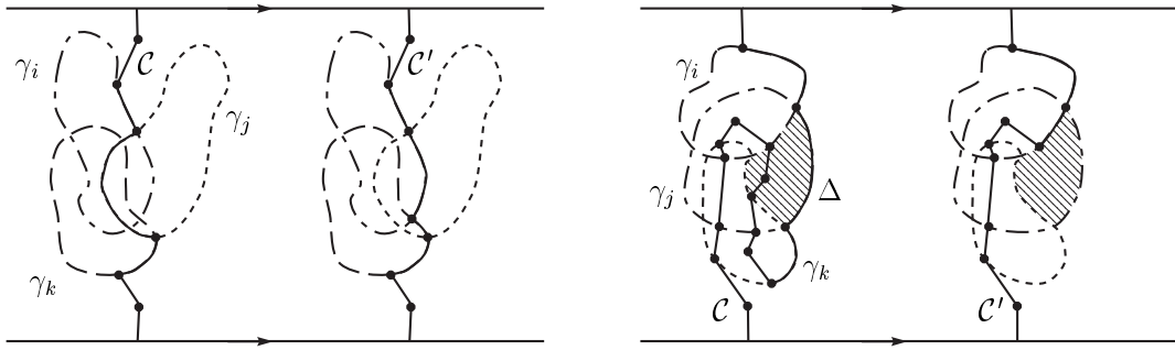
Fig. 6. Two examples for reducing the sequence.
