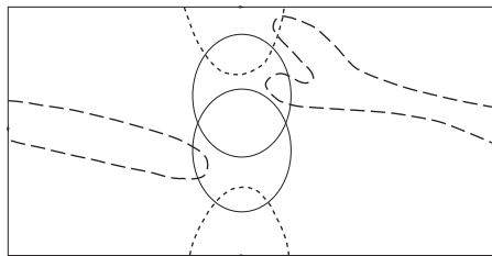
Fig. 3. An example illustrating Remark 9.
