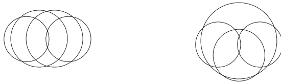
Fig. 2. An example illustrating Remark 7.
