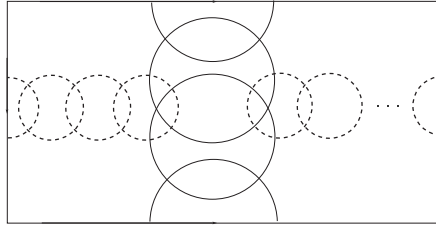
Fig. 16. A cellular generalised arrangement on the torus with all subarrangements embeddable into the sphere.
