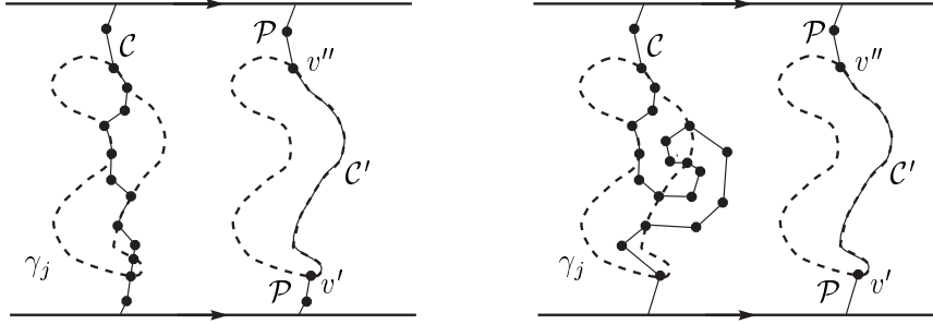
Fig. 5. Two examples for deleting multiple entries.
